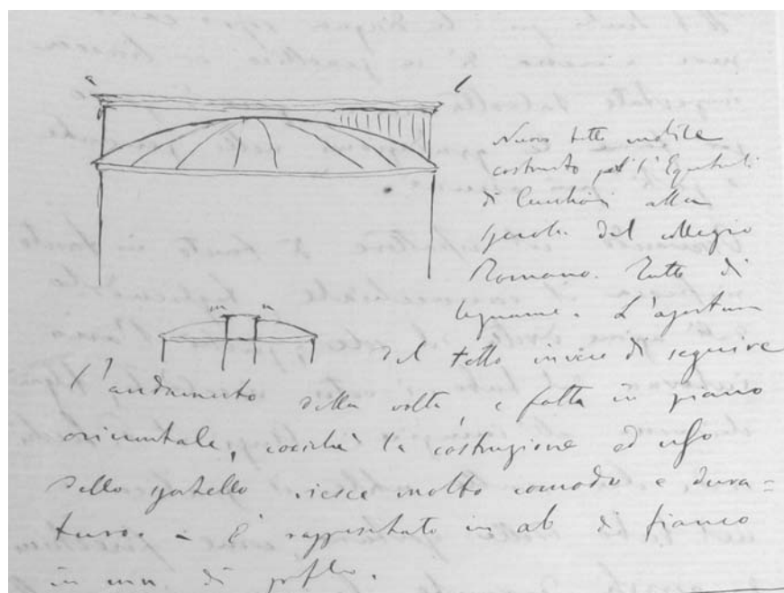
FIGURE 4 Sketch by Tacchini of the dome built for the Cauchy telescope at the Collegio Romano Observatory, which probably served as the model for the dome of the Palermo Merz equatorial (Archives of the INAF-Osservatorio Astronomico di Roma)
