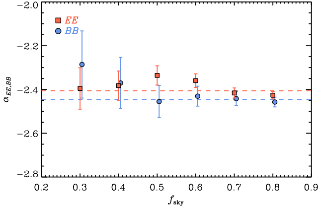
Fig. 3: Best-fit power-law exponents \alpha_{EE} (red squares) and \alpha_{BB} (blue circles) fitted to the 353 GHz dust \mathcal{D}_\ell^{EE} and \mathcal{D}_\ell^{BB} power spectra for the different LR regions defined in Sect. 3.3.1, distinguished here with f_{\text{sky}} . Although the values in the regions are not quite independent, simple means have been calculated and are represented as red and blue dashed lines.
