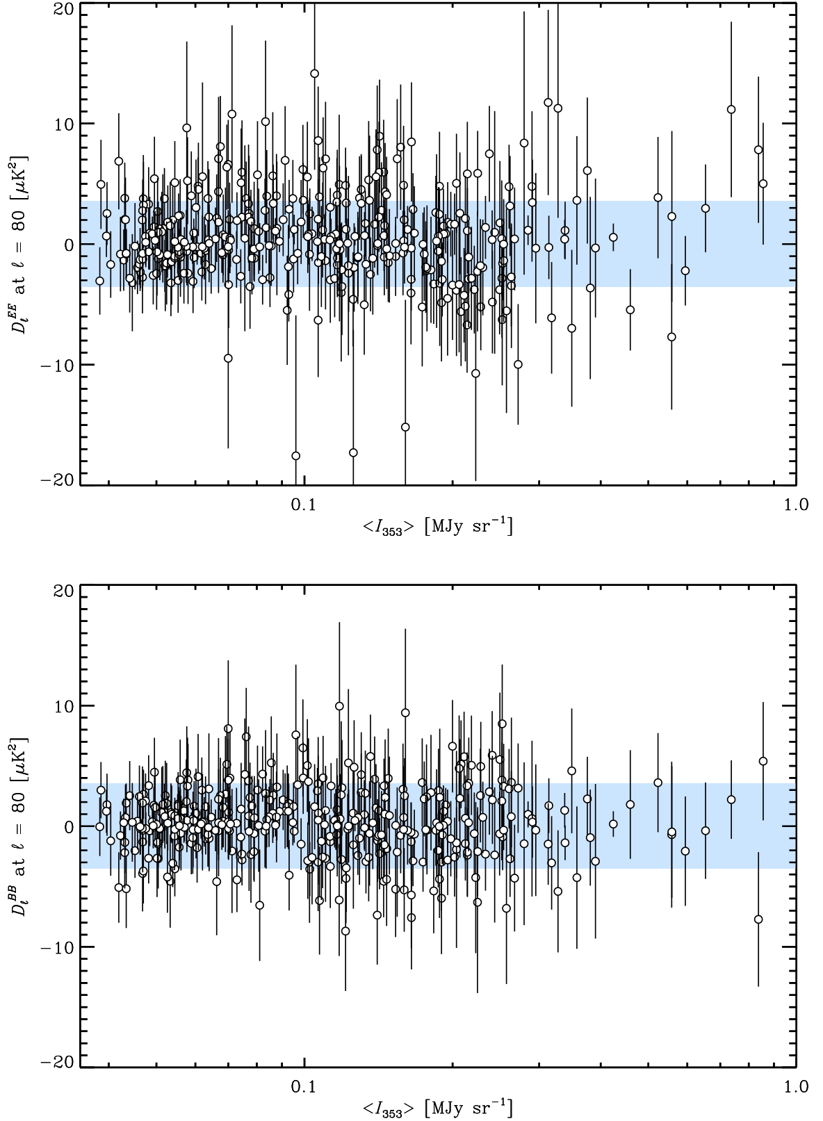
Fig. A.2: Top : same as Fig. 7, but instead of computing the \mathcal{D}_\ell^{EE} (top panel) and \mathcal{D}_\ell^{BB} (bottom panel) spectra from the 353 GHz cross-correlation between DetSet1 and DetSet2, we compute them from the cross-correlation between the HalfRing half-differences for each detector set, i.e., (353_{\text{DS1,HR1}} - 353_{\text{DS1,HR2}})/2 \times (353_{\text{DS2,HR1}} - 353_{\text{DS2,HR2}})/2 . The 3\sigma expectations from Planck inhomogeneous white-noise Monte Carlo simulations are represented as light-blue shaded areas.
