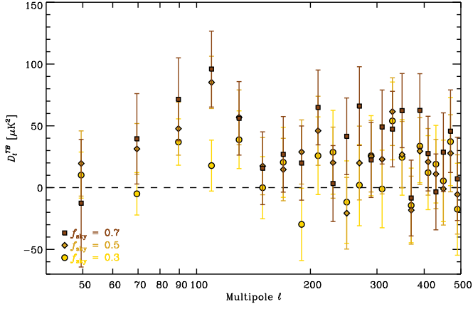
Fig. B.2: Planck HFI 353 GHz \mathcal{D}_\ell^{TB} power spectra (in \mu K_{\text{CMB}}^2 ) computed on three of the selected LR analysis regions that have f_{\text{sky}} = 0.3 (circles, lightest), f_{\text{sky}} = 0.5 (diamonds, medium), and f_{\text{sky}} = 0.7 (squares, darkest). The uncertainties plotted here are \pm 1 \sigma .
