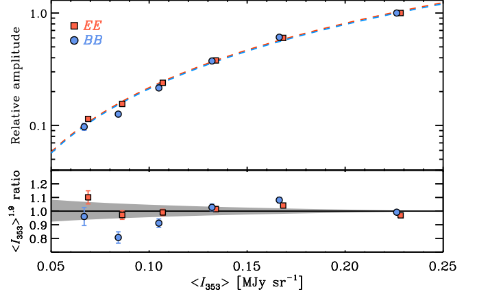
Fig. 4: Amplitude of the dust A^{EE} (red squares) and A^{BB} (blue circles) power spectra, normalized with respect to the largest amplitude for each mode. These are plotted versus the mean dust intensity \langle I_{353} \rangle for the six LR regions (top panel). A power-law fit of the form A^{XX}(\langle I_{353} \rangle) = K_{XX}\langle I_{353} \rangle^{1.9} , X \in \{E, B\} , is overplotted as a dashed line of the corresponding colour (these almost overlap). The bottom panel presents the ratio of the data and the fitted \langle I_{353} \rangle^{1.9} power law; the range associated with the \pm 1 \sigma uncertainty in the power-law exponent of 1.9 is displayed in grey. For details see Sect. 4.3.
