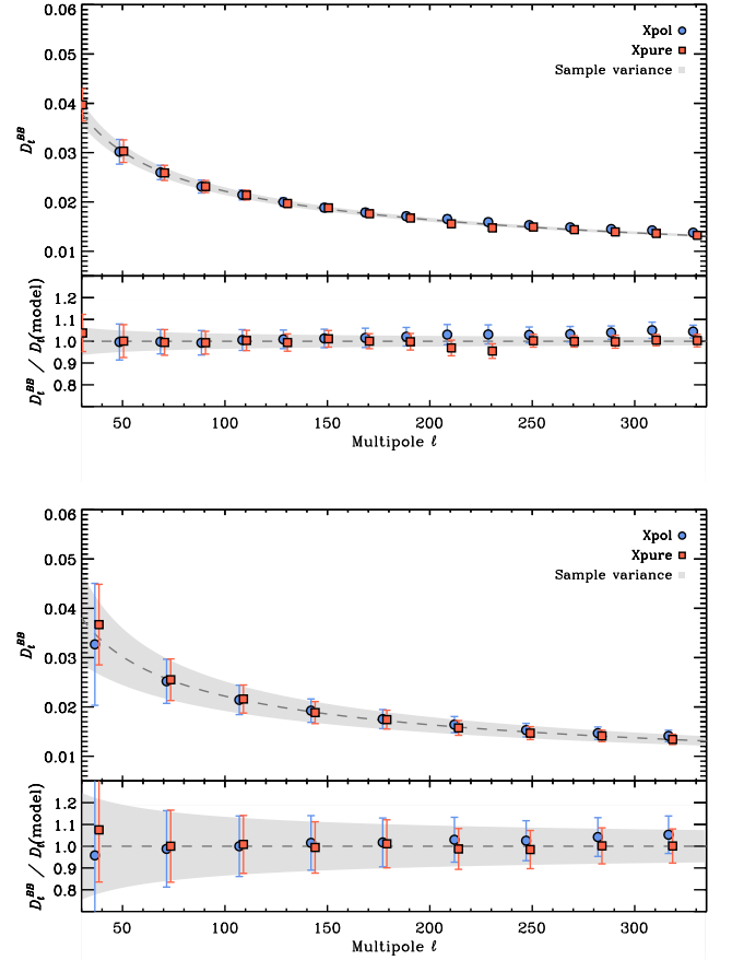
Fig. A.1: Upper parts of both panels: performance of the Xpol (blue points, see Sect. 3.1.1) and Xpure (red squares, see Sect. 3.1.2) algorithms on the \mathcal{D}_\ell^{BB} power spectrum for Gaussian simulations of the dust polarization in the LR24 region (top panel, defined in Sect. 3.3.1) and in M_{B2} (bottom panel, defined in Sect. 6.1). The signal input power spectrum is displayed as a dashed grey line and its associated sample variance as a light grey shaded area. Lower parts of both panels: relative discrepancy with respect to the input power spectrum.
