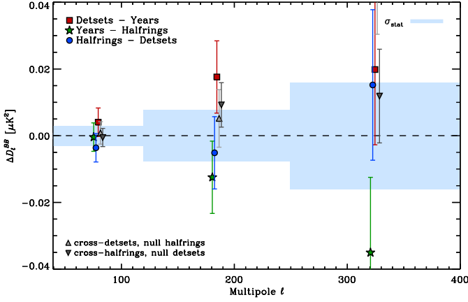
Fig. D.3: Planck 353 GHz \mathcal{D}_\ell^{BB} angular power spectrum differences extrapolated to 150 GHz, computed from the following cross-spectra differences: DetSets minus Years (red squares); Years minus HalfRings (green stars); and HalfRings minus DetSets (blue circles). We also show the null test performed using the cross-DetSets spectra of the HalfRing half-differences (light grey triangle) and the cross-HalfRings of the DetSet half-differences (dark grey reversed triangle) at 353 GHz. As in Fig. 9, the blue boxes represent the statistical uncertainties from noise; these are centred on zero, since we do not expect any signal for these null tests.
