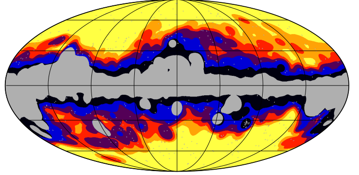
Fig. 1: Masks and complementary selected large regions that retain fractional coverage of the sky f_{\text{sky}} from 0.8 to 0.3 (see details in Sect. 3.3.1). The gray is the CO mask, whose complement is a selected region with f_{\text{sky}} = 0.8 . In increments of f_{\text{sky}} = 0.1 , the retained regions can be identified by the colours yellow (0.3) to black (0.8), inclusively. Also shown is the (unapodized) point source mask used.
