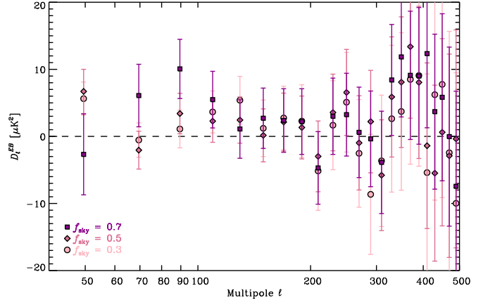
Fig. B.3: Planck HFI 353 GHz \mathcal{D}_\ell^{EB} power spectra (in \mu K_{\text{CMB}}^2 ) computed on three of the selected LR analysis regions that have f_{\text{sky}} = 0.3 (circles, lightest), f_{\text{sky}} = 0.5 (diamonds, medium), and f_{\text{sky}} = 0.7 (squares, darkest). The uncertainties plotted here are \pm 1 \sigma .
