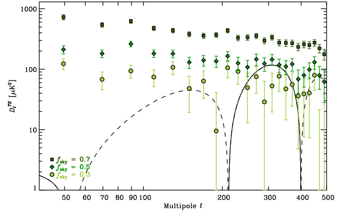
Fig. B.1: Planck HFI 353 GHz \mathcal{D}_\ell^{TE} power spectra (in \mu\text{K}_{\text{CMB}}^2 ) computed on three of the selected LR analysis regions that have f_{\text{sky}} = 0.3 (circles, lightest), f_{\text{sky}} = 0.5 (diamonds, medium), and f_{\text{sky}} = 0.7 (squares, darkest). The uncertainties plotted here are \pm 1\sigma . The Planck 2013 best-fit \Lambda\text{CDM} \mathcal{D}_\ell^{TE} expectation (Planck Collaboration XVI 2014) is displayed as the black curve, solid where positive, dashed where negative.
