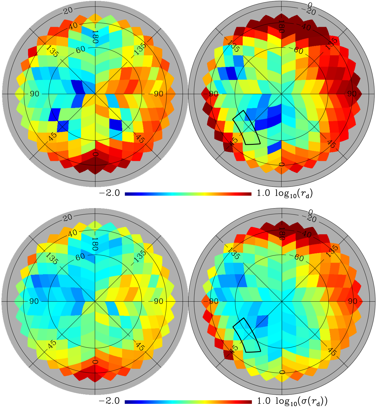
Fig. 8: Top : map in orthographic projection of the 150 GHz \mathcal{D}_\ell^{BB} amplitudes at \ell = 80 , computed from the Planck 353 GHz data, extrapolated to 150 GHz, and normalized by the CMB expectation for tensor-to-scalar ratio r = 1 . The colours represent the estimated contamination from dust in r_d units (see details in Sect. 5.3). The logarithm of the absolute value of r_d for a 400 \text{ deg}^2 patch is presented in the pixel on which the patch is centred. As described in Sect. 3.3.2, the patches overlap and so their properties are not independent. The northern (southern) Galactic hemisphere is on the left (right). The thick black contour outlines the approximate BICEP2 deep-field region (see Sect. 6). Bottom : associated uncertainty, \sigma(r_d) .
