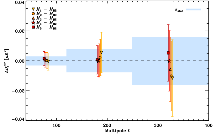
Fig.D.2: Planck 353 GHz \mathcal{D}_\ell^{BB} angular power spectrum differences extrapolated to 150 GHz, determined from the spectra computed on the M_{1-5} regions presented in Appendix D.2 and the spectrum computed on M_{B2} . \mathcal{D}_\ell^{BB} difference values for the five regions are displayed using colours from yellow (for M_1 ) to dark red (for M_5 ). As in Fig. 9, the blue boxes represent the statistical uncertainties from noise associated with the M_{B2} spectrum. They are centred on zero, since we compute spectrum differences here.
