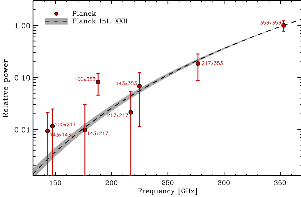
Fig. 10: Frequency dependence of the amplitude A^{BB} of the angular power spectrum \mathcal{D}_\ell^{BB} computed on M_{B2} defined in Sect. 6.1, normalized to the 353 GHz amplitude (red points); amplitudes for cross-power spectra are plotted at the geometric mean frequency. The square of the adopted dust SED, a modified blackbody spectrum with \beta_d = 1.59 and T_d = 19.6 K, is over-plotted as a black dashed-line, again normalized to the 353 GHz point. The \pm 1\sigma error area arising from the expected dispersion of \beta_d , 0.11 for the M_{B2} patch size (Sect. 2.2.1), is displayed in light grey.
