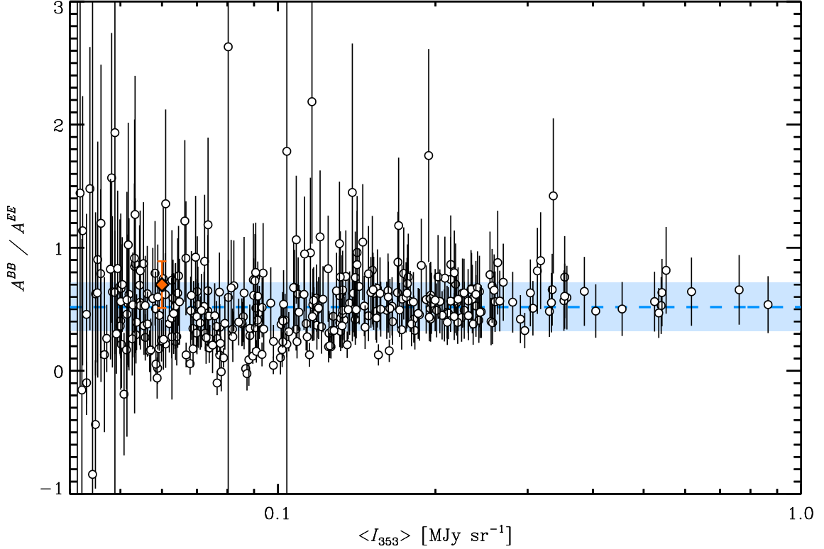
Fig. A.3: Ratio of the dust A^{BB} and A^{EE} angular power spectra amplitudes computed on the 352 patches at high Galactic latitudes (described in Sect. 5, circles), as a function of the mean dust intensity \langle I_{353} \rangle of the patch. The mean value, \langle A^{BB}/A^{EE} \rangle = 0.51 \pm 0.18 here, is represented as a dashed-blue line and the associated \pm 1\sigma dispersion as a light blue shaded area. The A^{BB}/A^{EE} ratio for the M_{B2} spectra presented in Sect. 6.3 is displayed as an orange diamond.
