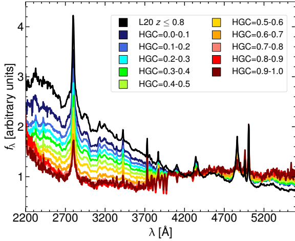
Fig. 10. Comparison between the stacks in bins of HGF and our reference spectrum (black) for the z \leq 0.8 interval, as colour-coded in the legend. All the spectra are scaled to their 4200 Å flux. Increasingly host-dominated composites exhibit flatter UV continua.
