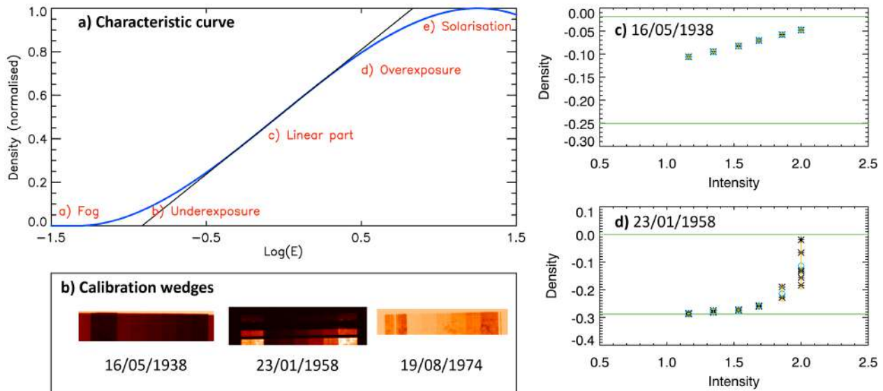
Figure 5. a) Schematic of a characteristic curve of photographic observations (blue) and a linear fit (black) to the central part of the curve. b) Examples of calibration wedges from the Arcetri observatory. c-d) Characteristic curves determined from the first two Arcetri calibration wedges shown in panel b). Black asterisks show individual measurements from the wedges, blue circles the mean density value for each intensity value, while yellow marks the symmetric 1\sigma interval. The green horizontal lines denote the minimum and maximum values found within the solar disc for each day.
