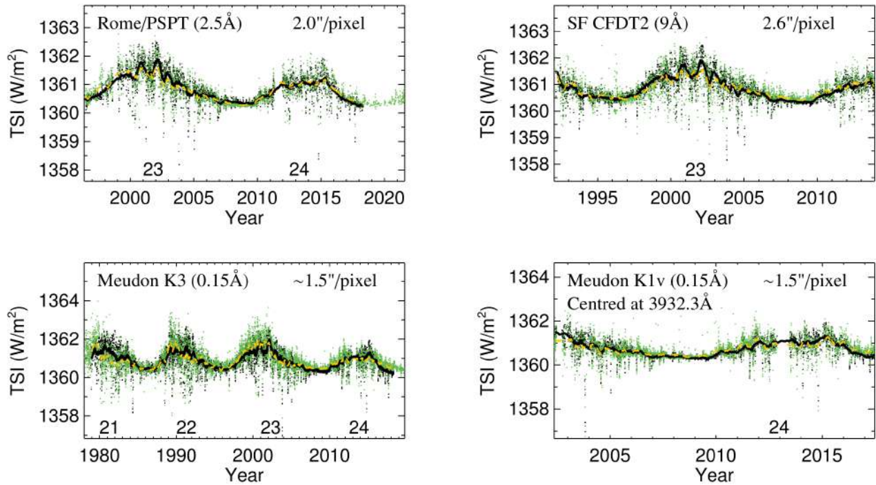
Figure 13. Reconstructed TSI series by Chatzistergos et al. (2021a) with Ca II K data from Rome/PSPT, San Fernando CFDT2, Meudon K3, and Meudon K1v. The reconstructions are shown in green dots for daily values and dashed yellow for 81-day running means. Also shown is the PMOD TSI composite (black dots for daily values and black line for 81-day running mean values). The numbers at the lower part of the figures denote the conventional solar cycle numbering. Also listed within the figures are the bandwidth used for the observations as well as the pixel scale (for Meudon K1v we also list the central wavelength).
