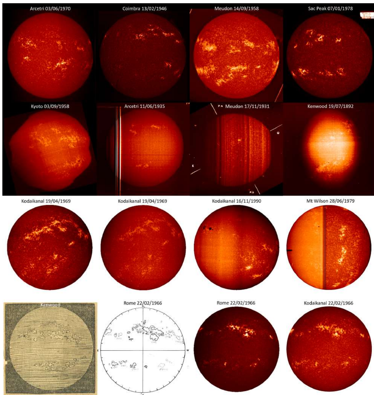
Figure 2. Exemplary raw full-disc images of the Sun in the Ca II K line. The first row shows images of good quality from four historical photographic archives, indicated at the top of each image together with the date of observation. The next three rows aim at highlighting some characteristics of such data. In particular, the second row shows image distortions due to spectroheliograph problems, while the third row showcases visual differences due to variations in central wavelength or bandpass used for observations. The last row shows Ca II K drawings from Kenwood and Rome observatories as compared to a filtergram and spectroheliogram from Rome and Kodaikanal taken on the same day as the Rome drawing.
