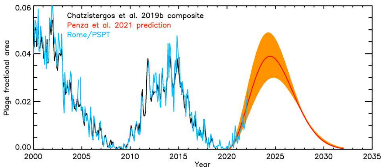
Figure 11. Prediction of solar cycle 25 amplitude in plage fractional areas by Penza et al. (2021, red, with confidence intervals in shaded orange surface). Shown also is the Chatzistergos et al. (2019b) plage area composite (black), on which the prediction was based, as well as more recent data from Rome/PSPT (light blue), which was the reference observatory in the Chatzistergos et al. (2019b) plage area composite since 1996.
