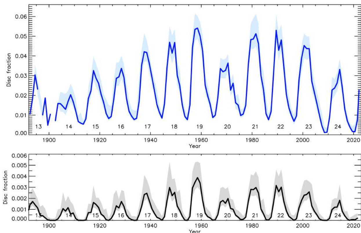
Figure 10. Top: Plage area composite series by Chatzistergos et al. (2020c) extended to 10 March 2022 with Rome/PSPT data processed in the same way as the rest of the data used for the composite series. Bottom: Sunspot area series by Mandal et al. (2020). Shaded areas mark the asymmetric 1\sigma intervals, while the numbers at the lower part of each panel denote the conventional solar cycle numbering.
