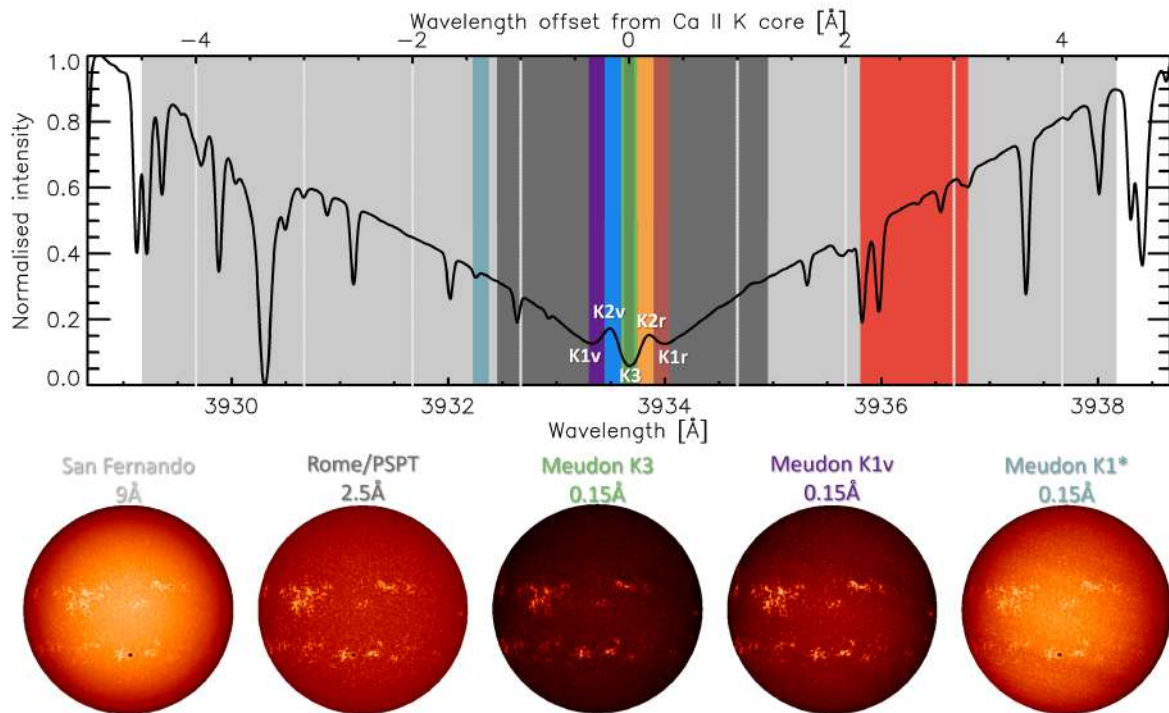
Figure 4. The normalised high-resolution disc-integrated solar spectrum over a 10\text{\AA} interval centred at the core of the Ca II K line from the atlas of the Hamburg Observatory. Also shown are the nominal pass-bands of selected Ca II K archives, including the two extreme cases from San Fernando (light grey) and Meudon K3 (light green up to 2017, darker green since 2017), an average case for CCD-based archives from the Rome/PSPT (dark grey), along with six off-band archives: MLSO/PSPT (red), Meudon K2r (orange), K1r (brown), K2v (blue), K1v (purple), and Meudon K1* (light blue, this is referred to as K1 in the Meudon database even though it is not at the K1 minimum, but centred further away at the wing of the line at 3932.3\text{\AA} ). The vertical light grey lines mark wavelength intervals of 1\text{\AA} from the core of the Ca II K line. The bottom part of the figure presents five exemplary observations taken on the same day (2013/09/23) at San Fernando, Rome/PSPT, Meudon K3, Meudon K1v, and Meudon K1*.
