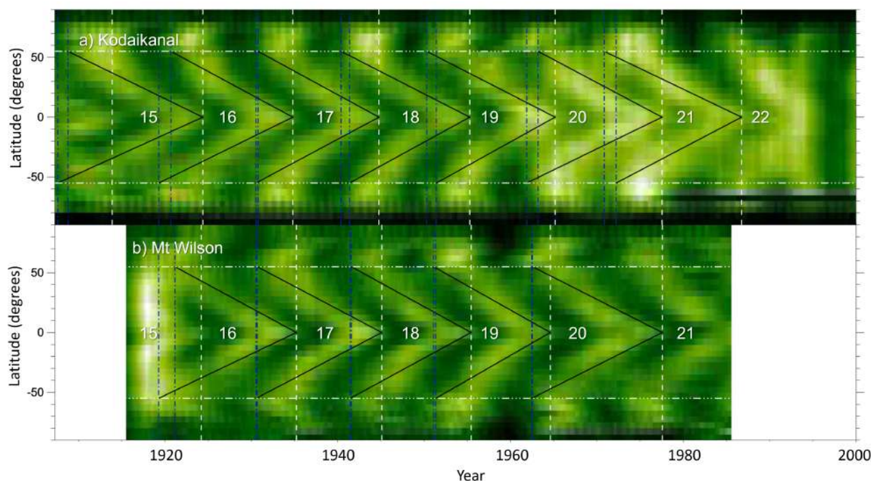
Figure 12. Time-latitude maps of network areas from Kodaikanal (top panel) and Mt Wilson (bottom) observatories. The black lines are fits to the extended equatorward branches. The vertical dashed blue lines denote the onset of the extended equatorward branches, while the white vertical dashed lines denote the time when those branches reach the equator. The horizontal white dashed lines mark latitudes at \pm 55^\circ . The numbers at the centre of each panel denote the conventional solar cycle numbering. The figure is adapted from Chatterjee et al. (2019)
