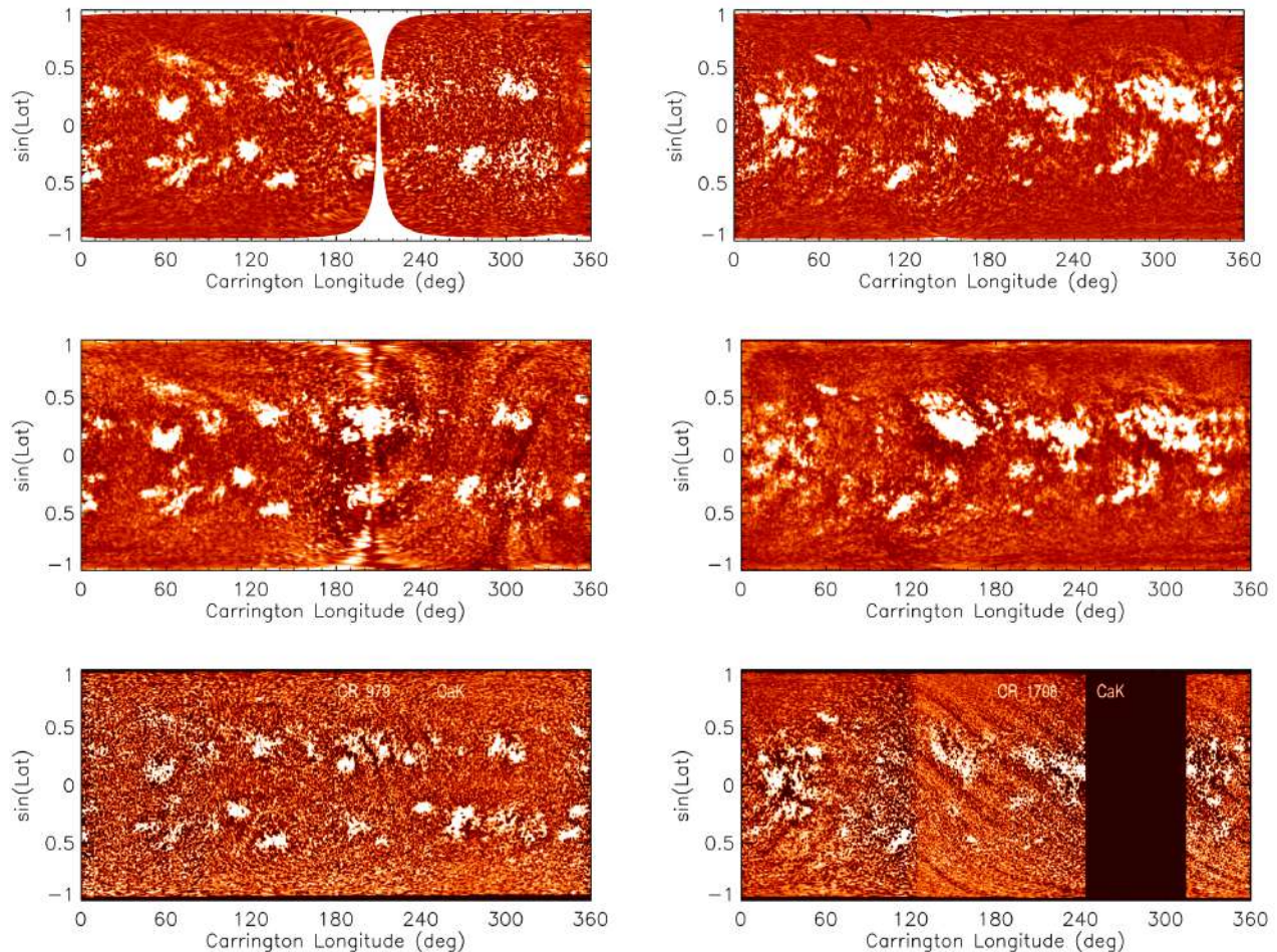
Figure 8. Examples of Carrington maps constructed from Ca II K data over rotations 979 (23/11–19/12/1926, left) and 1708 (2/5–29/5/1981, right). Shown are Mt Wilson data processed by Chatzistergos et al. (2020c, top panel) and by Bertello et al. (2020, middle panel) as well as Kodaikanal data processed by Chatterjee et al. (2016, bottom panel). Due to differences in the image processing the images are saturated at different levels in order to show plage at roughly similar levels. In particular, the contrast ranges are [-0.2-0.2] and [-0.5-0.5] for the first and second rows, respectively, while the 3rd row shows images to their entire range. The data by Chatterjee et al. (2016) are provided in PNG file format so the exact contrast values are not known to us.
