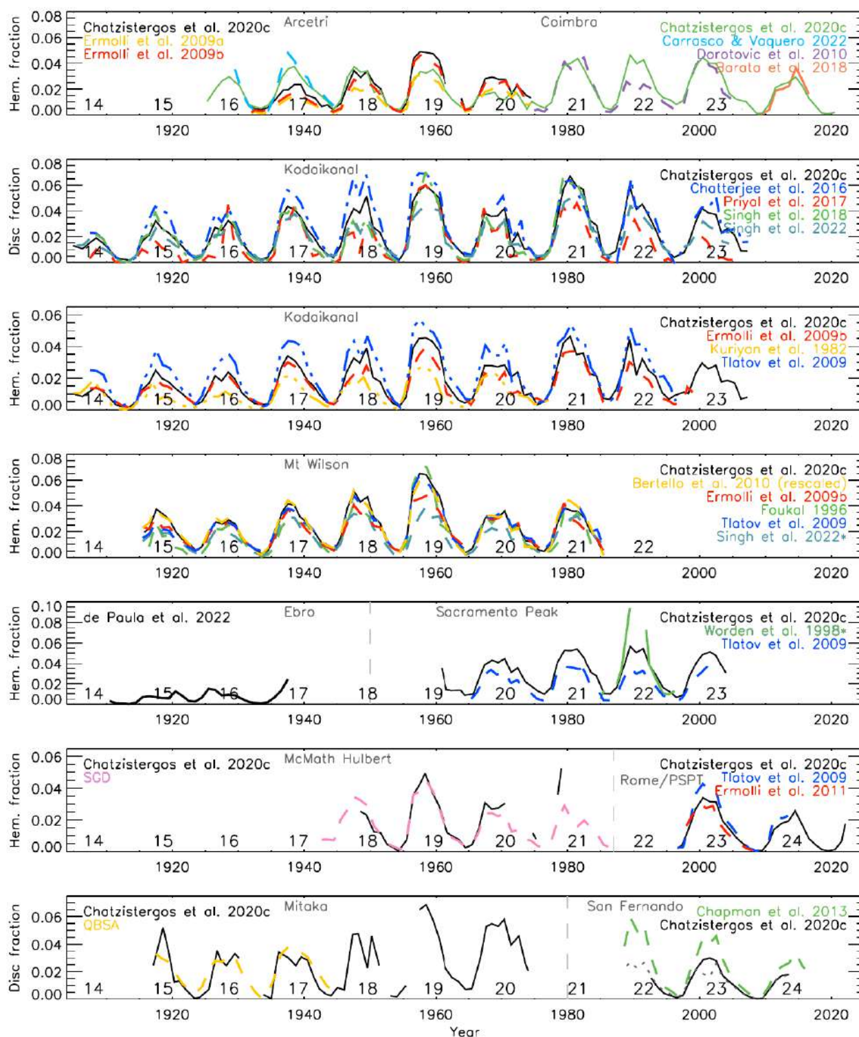
Figure 9. Plage areas derived from various Ca II K archives (as indicated in grey) and different studies. For the San Fernando series by Chatzistergos et al. (2020c) we show separately the results for CFDT1 (dotted grey) and CFDT2 (black) data. Shown are annual median values in hemispheric fraction, except for the series in 2nd and 7th rows as well as the one by Singh et al. (2022) in the 4th row and Worden et al. (1998a) in the 5th row which are given in disc fraction. The numbers in the lower part of each panel denote the conventional solar cycle numbering. The vertical lines roughly mark the separation of archives in panels including timeseries from more than one archive.
