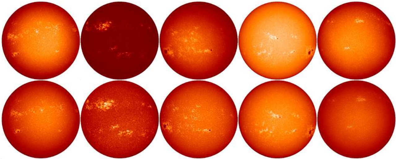
Figure 6. Examples of amateur Ca II K observations (bottom row) along with co-temporal images from professional observatories (top row). From left to right, the images were taken on 24/12/2015, 21/04/2022, 19/10/2014, 28/10/2014, and 13/02/2010 by the amateur observers (top): Michael Borman, Didier Favre, André Gabriël, Lastrofieffe, Stefano Sello, and at professional observatories (bottom): Kanzelhöhe, Meudon, Valašské Meziříčí, Calern, and Pic du Midi.
