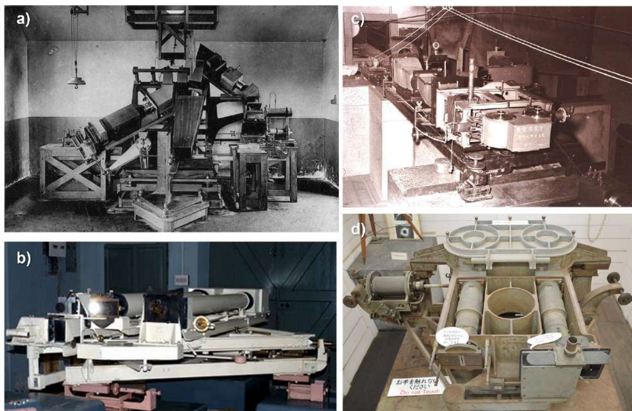
Figure 3. Spectroheliographs used at the observatories of Meudon (panel a; https://www.observatoiredeparis.psl.eu/the-meudon-spectroheliograph.html?lang=en , Kodaikanal (panel b; https://kso.iiap.res.in/new/instruments , Mitaka (panel c; https://solarwww.mtk.nao.ac.jp/en/topics/topics_0001.html , and Kyoto (panel d; photo taken by T. Chatzistergos).
