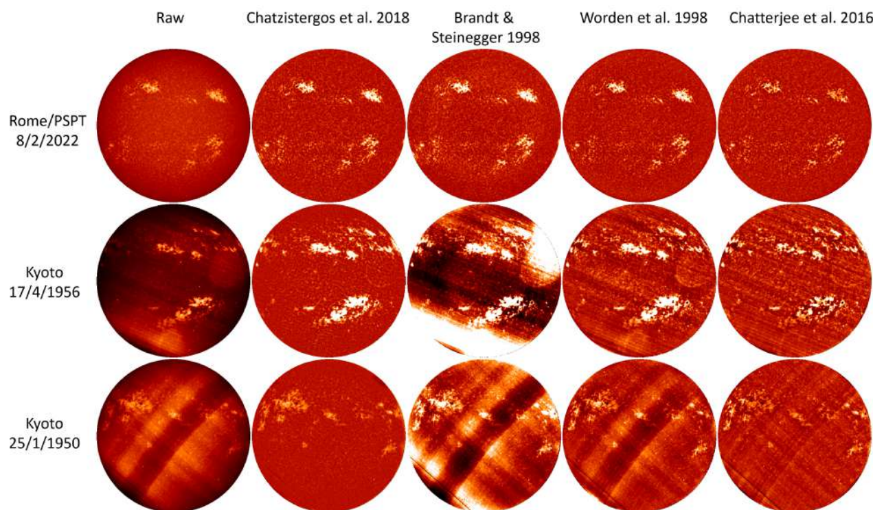
Figure 7. Examples of the performance of selected methods to compensate for the limb darkening on observations from Rome/PSPT (8 February 2022; top row) and Kyoto observatory (17 April 1956 in the middle row and 25 January 1950 in the bottom row). Raw images (i.e. including the limb darkening and image artefacts) are shown in the left column. Columns 2–5 show images compensated for the limb-darkening with the methods by Chatzistergos et al. (2020c), Brandt and Steinegger (1998), Worden et al. (1998a), and Chatterjee et al. (2016), respectively. Raw images are shown to their full intensity range, while the limb darkening-compensated images are shown in the range [-0.5-0.5] in contrast.
