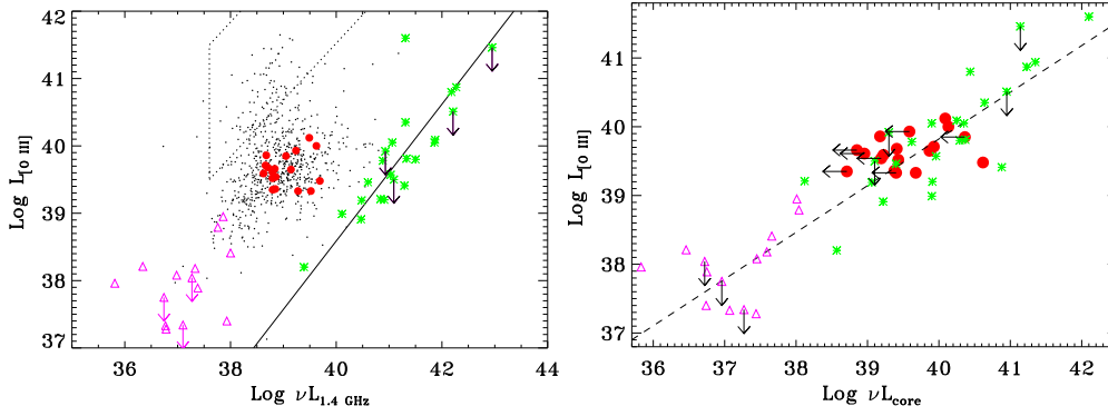
Fig. 9 Left panel: NVSS vs. [O III] line luminosity ( \text{erg s}^{-1} ). The small points correspond to the SDSS/NVSS sample selected by Best and Heckman (2012). The solid line represents the correlation between line and radio luminosity derived for the 3C/FR I sample (green stars) (Baldi et al., 2019a). The dotted lines include the region where RQAGN (Seyferts) are found. The filled circles are FR 0s studied with the VLA by Baldi et al. (2019a) and the empty pink triangles are the CoreG. Right panel: VLA radio core vs [O III] line luminosity ( \text{erg s}^{-1} ) for 3C/FR Is, FR 0s and CoreG and the dashed line represents their common radio-optical luminosity correlation.
