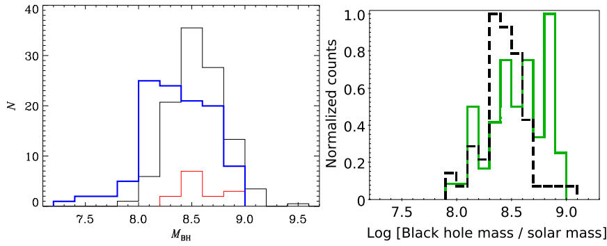
Fig. 3 Left panel: BH mass distribution (in M_{\odot} ) of FR 0s (FR0CAT, blue line) with respect to FR 1s (FRICAT, radio size > 30 kpc, black line) and small FR 1s (sFRICAT, 10 < \text{radio size} < 30 kpc, red line) from Baldi et al. (2018). Right panel: compact (black) and extended RGs (green) from Miraghaei and Best (2017), when matched in radio core luminosities.
