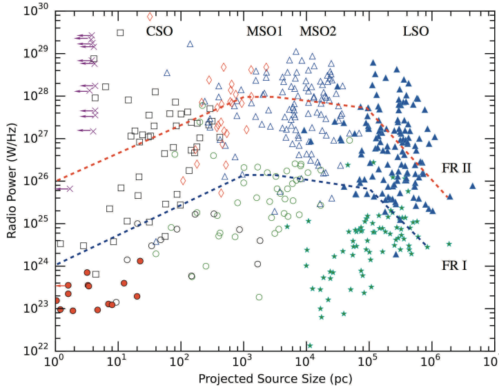
Fig. 18 Radio power vs. source size (P-D diagram) of RGs taken from Cheng and An (2018) and An and Baan (2012) . Black squares are CSO, black circles are low-power GPSs, red diamonds are high-power GPSs, purple crosses are HFPs, green circles are low-power CSSs, blue open triangles are high-power CSSs, blue filled triangles are FR IIs, and green filled stars are FR Is. A further morphological sub-classification is also considered that distinguishes among CSO ( < 1 kpc), MSO (1–15 kpc), and large symmetric objects (LSO; > 15 kpc, FR I/II) ( Readhead, 1995 ). Red and blue dashed lines are illustrative of the evolutionary tracks based on parametric modeling for the high-power and low-power sources, respectively. The pc-scale FR 0s (red filled circles) studied by Cheng and An (2018) are situated in the bottom-left corner, occupied by low-power CSOs and some compact low-power MSOs.
