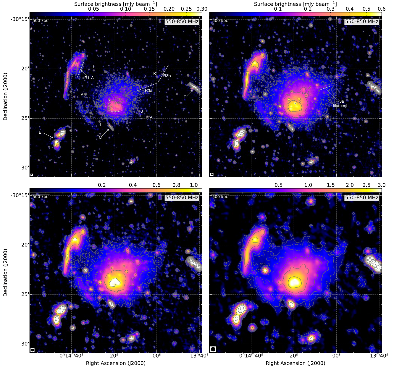
Fig. 3. Total power uGMRT (550–850 MHz) images of Abell 2744 at different resolutions (5'', top left ; 10'', top right ; 15'', bottom left ; 25'', bottom right ). The known diffuse emission sources, namely the main relic (R1), the fainter relics (R2, R3, and R4), and the extended halo are recovered in our new uGMRT observations. The radio emission at the center of the halo apparently shows a cone-like morphology. The image properties are given in Table 2. Here, panel top left, top right, bottom left and bottom right correspond to IM9, IM10, IM12, and IM15, respectively. Contour levels are drawn at [1, 2, 4, 8, \dots] \times 3.5 \sigma_{\text{rms}} . In these images there is no region below -3 \sigma_{\text{rms}} . The beam size is indicated in the bottom left corner of the each image.
