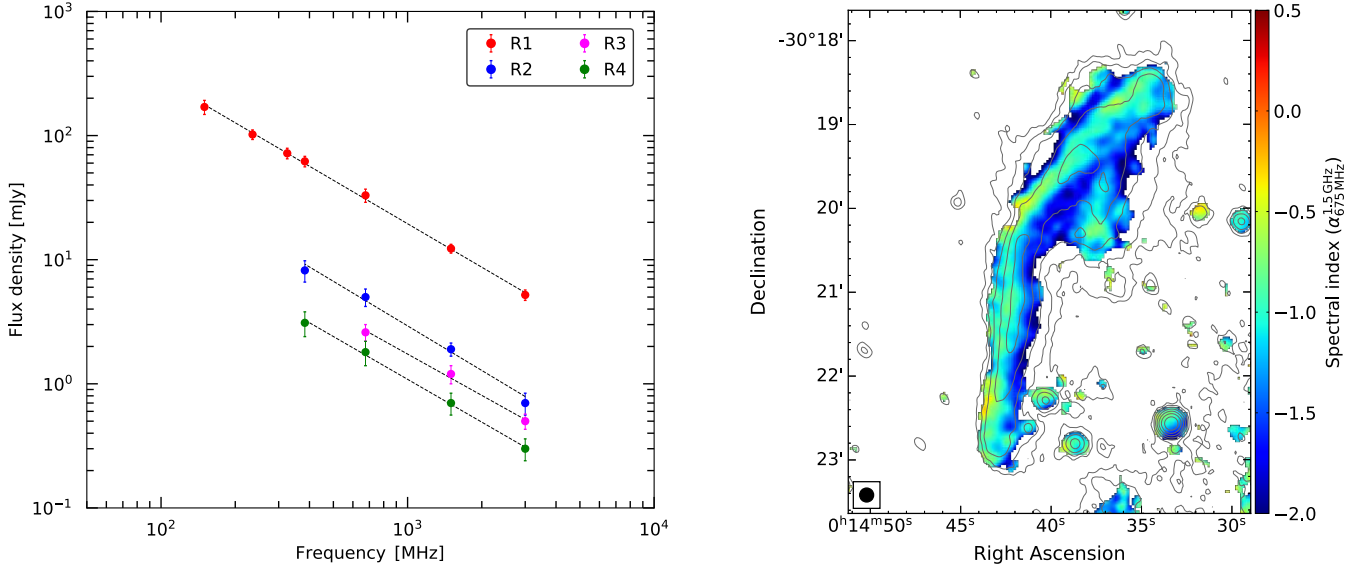
Fig. 7. Left: integrated radio spectra of relics R1, R2, R3, and R4. Dashed lines are the fitted power-law with indices given in Table 3. Regions used to obtain the integrated flux densities of all four relics are shown in the right panel of Fig. 7. Right: spectral index map of the main relic R1 between 675 MHz and 1.5 GHz at 10'' resolution (corresponding to IM6 and IM11 in Table 2), showing a clear spectral index gradient across the entire relic. Contour levels are drawn at [1, 2, 4, 8, \dots] \times 3.5 \sigma_{\text{rms}} , and are from the uGMRT Band 4 image.
