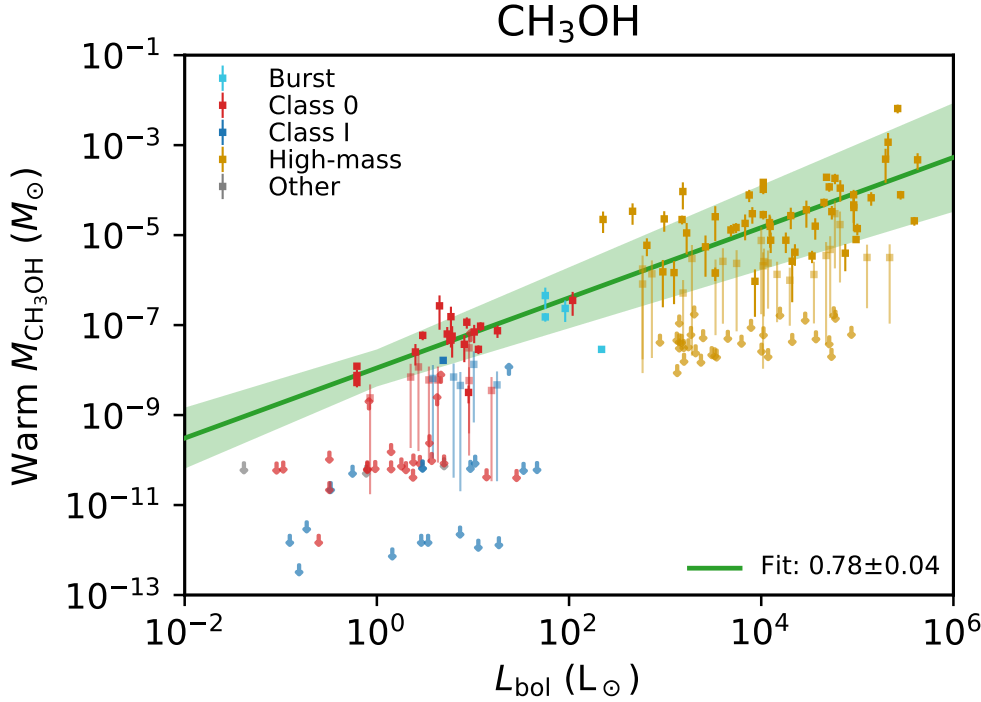
Fig. 3. Warm \text{CH}_3\text{OH} mass as a function of the bolometric luminosity. Different colors denote different observational classes, and all sources with L_{\text{bol}} > 1000 L_{\odot} are classified as high-mass sources. Additionally, sources that are suggested to currently be in a burst phase (e.g., V883 Ori and IRAS 2A; van 't Hoff et al. 2018; Lee et al. 2019b; Hsieh et al. 2019) are highlighted. Sources in the “other” category include Class II and flat spectrum sources. The green line indicates the best-fit power-law model to the data points (excluding the upper limits) and the green shaded area the 3\sigma uncertainty on the fit.
