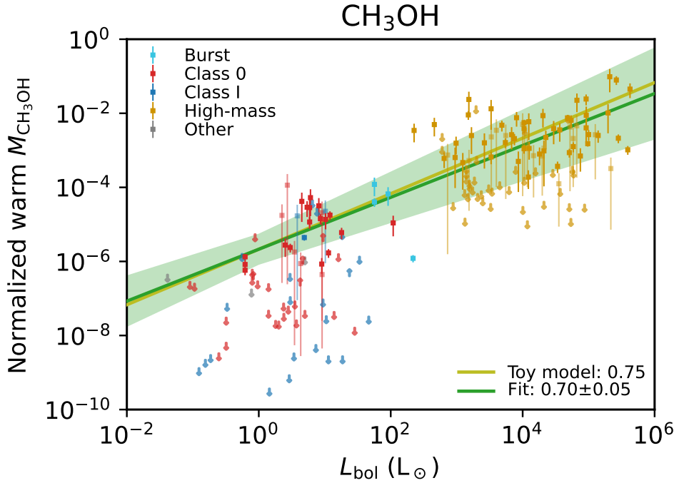
Fig. 4. Normalized warm gaseous CH 3 OH mass, M_{\text{CH}_3\text{OH}}/M_{\text{dust},0} , as a function of the bolometric luminosity. Different colors denote different observational classes, and all sources with L_{\text{bol}} > 1000 L_{\odot} are classified as high-mass sources. Additionally, sources that are suggested to currently be in a burst phase (e.g., V883 Ori and IRAS2A; van ’t Hoff et al. 2018; Lee et al. 2019b; Hsieh et al. 2019) are highlighted. Sources in the “other” category include Class II and flat spectrum sources. The green line indicates the best-fit power-law model to the data points (excluding the upper limits) and the green shaded area the 3\sigma uncertainty on the fit. The yellow line indicates the relation for the toy model of Eq. (4) scaled to match the best-fit power-law model.
