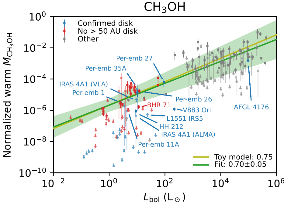
Fig. 5. Normalized warm gaseous \text{CH}_3\text{OH} mass with respect to M_{\text{dust}} within a 200 au radius as a function of the bolometric luminosity. Sources around which a disk has been detected on >10 au scales are indicated in blue, and sources where no disk is confirmed on >50 au scales are indicated in red. All other sources (i.e., with no information about a disk) are shown in gray. The green line indicates the best-fit power-law model to the data points (excluding the upper limits) and the green shaded area the 3\sigma uncertainty on the fit. The yellow line indicates the relation for the toy model of Eq. (4) scaled to match the best-fit power-law model.
