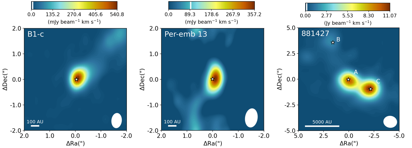
Fig. 1. Integrated intensity maps of the CH 3 OH 2 1,1 -1 0,1 line for the low-mass protostar B1-c ( left ), the CH 3 OH 5 1,4 -4 1,3 line for the low-mass protostar Per-emb 13 from PEACHES ( middle ), and the CH 3 OH 8 0,8 -7 1,6 line for the high-mass 881427 cluster ( right ). The color scale is shown on top of each image. The images are integrated over [-5,5] km s -1 with respect to the V_{\text{lsr}} . The peaks in the continuum are indicated with the white stars. The white ellipse in the lower right of each image depicts the beam size, and in the lower left a physical scale bar is displayed.
