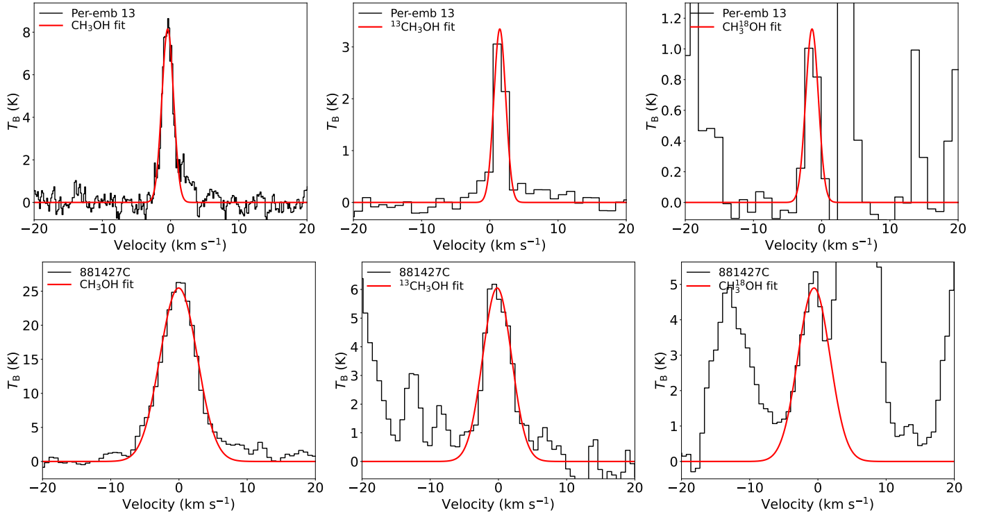
Fig. 2. Spectral line fits of CH 3 OH ( left ), 13 CH 3 OH ( middle ), and CH 3 18 OH ( right ) for Per-emb 13 from the PEACHES sample ( top row ) and 881427C from the ALMAGAL sample ( bottom row ). The data corrected for the V_{lsr} are shown in black, and the fit for T_{ex} = 150 K is shown in red. All lines are >3\sigma detections. The top row shows the CH 3 OH 5_{1,4}-4_{1,3} ( E_{up} = 50 K), 13 CH 3 OH 23_{3,20}-23_{2,21} ( E_{up} = 675 K), and CH 3 18 OH 11_{2,10}-10_{3,7} ( E_{up} = 184 K) lines, and the bottom row shows the CH 3 OH 8_{0,8}-7_{1,6} ( E_{up} = 97 K), 13 CH 3 OH 14_{1,13}-13_{2,12} ( E_{up} = 254 K), and CH 3 18 OH 8_{1,8}-7_{0,7} ( E_{up} = 86 K) lines.
