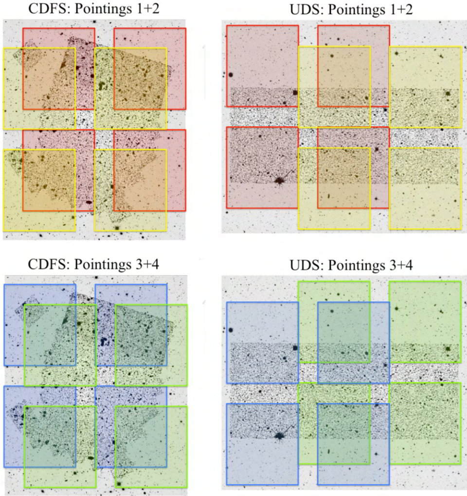
Fig. 1. Layout of the VANDELS pointings, from McLure et al. (2018) Fig. 1. Left: CDFFS, right: UDS; north is up and east to the left. Each area is shown twice to better show the layout of the four VIMOS pointings (coloured squares). The greyscale image shows the HST H -band imaging provided by the CANDELS survey ( Koekemoer et al. 2011 ; Grogin et al. 2011 ) in the central regions and the ground-based H -band imaging from UKIDSS UDS ( Almaini et al., in prep. ) and VISTA VIDEO ( Jarvis et al. 2013 ) in the wider region.
