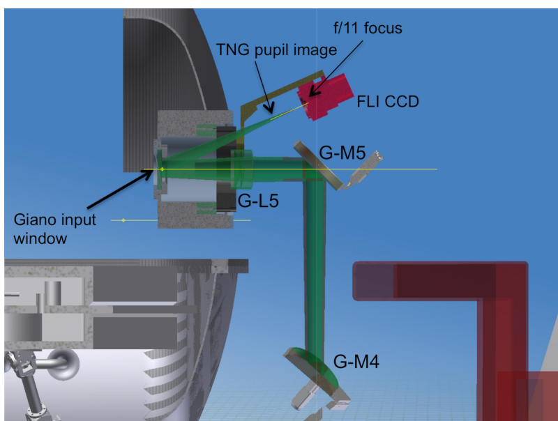
Figure 9 Guider placed on the reflected beam of Giano input window.
