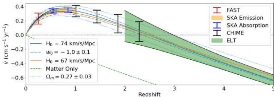
Fig. 47 Forecast acceleration measurements versus redshift for the SKA using H \text{i} 21-cm emission from galaxies (Kloekner et al. 2015), CHIME using H \text{i} 21-cm absorption (Yu et al. 2014), H \text{i} 21-cm absorption using FAST and the SKA estimated from projected detections (see text), and an ELT program that monitors the Ly \alpha forest (Liske et al. 2008). The cosmological tracks follow Fig. 46. The shaded loci and error bars indicate 1\sigma uncertainties
