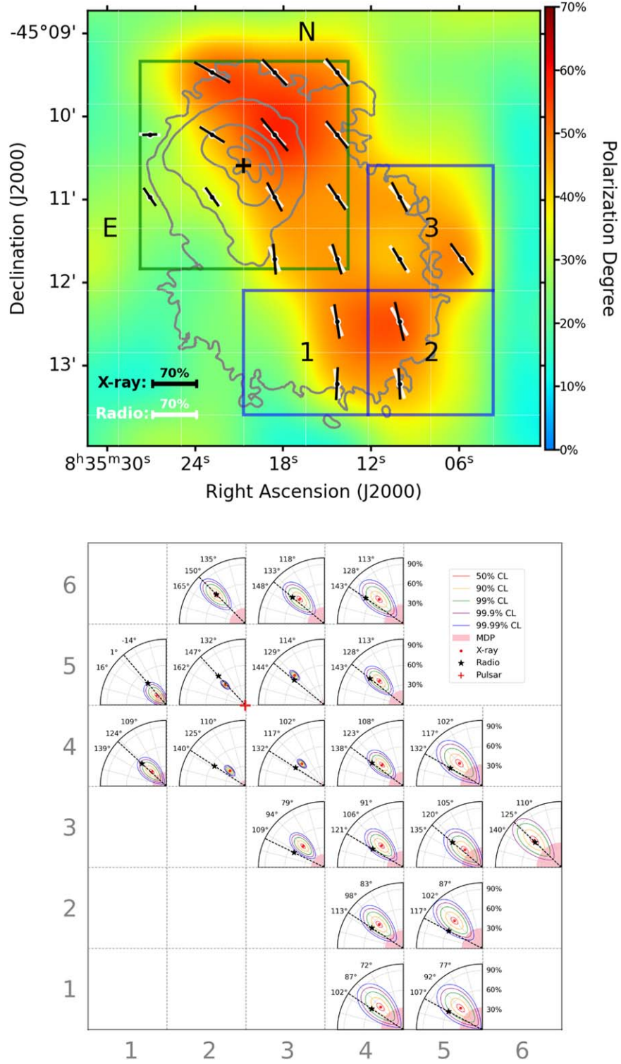
Figure 2. (Top) The PD map of the Vela PWN in the 2–5 keV energy range with a pixel size of 45'' overlaid with the Chandra contour. Pixels with X-ray PD > MDP_{99} have polarization vectors on top. The length of the black (white) lines indicates the PD measure in X-ray (radio), and orientation indicates the projected magnetic field. (Bottom) The polarization protractor plot for pixels with the polarization vector overlaid on the top panel, covering the same region, with radius and polar angle indicating the PD and PA, respectively.
