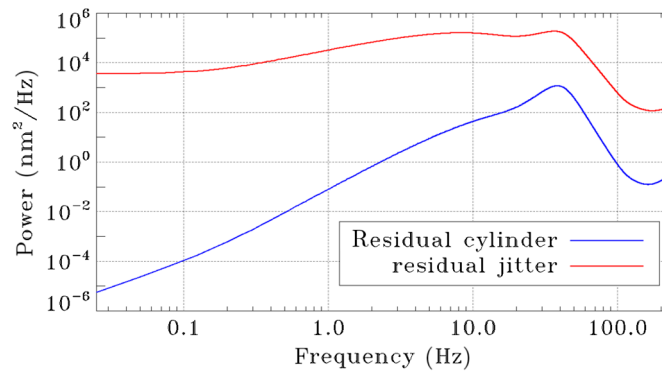
Fig. 7 PSDs of the input residual LGS jitter and of the rolling shutter-induced cylinder after propagation into the AO loop.
