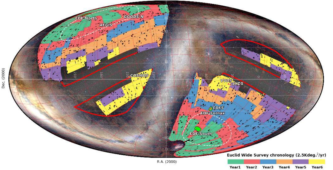
Fig. 46. RSD 2021A (14 514 deg 2 ) chronology shown in celestial coordinates. RoI boundaries are shown as solid red lines. Blinding stars cause 809 avoidance areas within the reference survey, with an average of 0.785 deg 2 per avoidance area, totalling 635 deg 2 . Dashed lines (1300 deg 2 in white per Galactic cap) delimit the highest S/N areas. The ecliptic referential is over-plotted in red. The three EDFs (bright green) and the six EAFs (red diamonds, not to scale) are shown.
