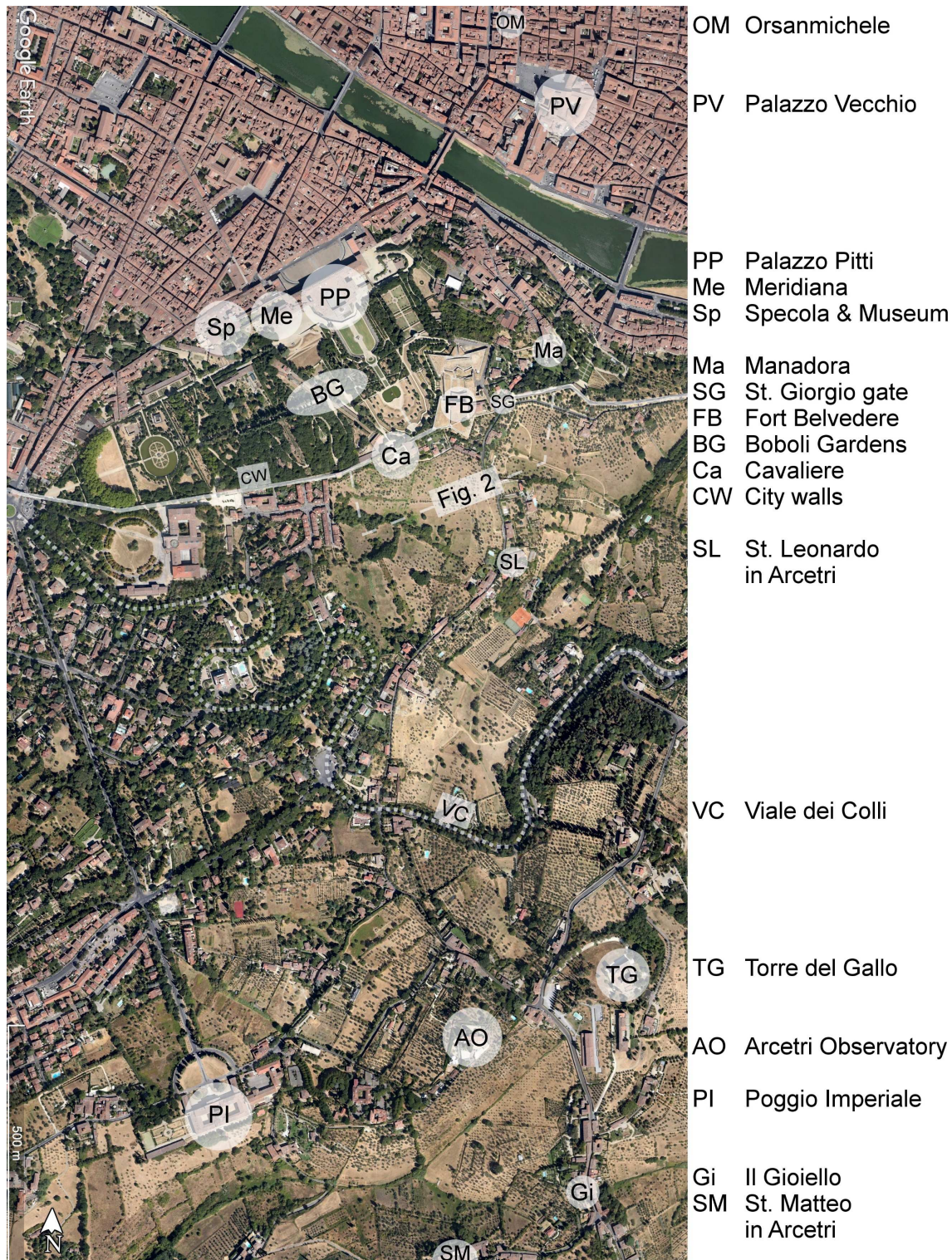
Figure 1: Aerial view of Florence from the city centre in the north to the Arcetri area in the south (Google Earth).
