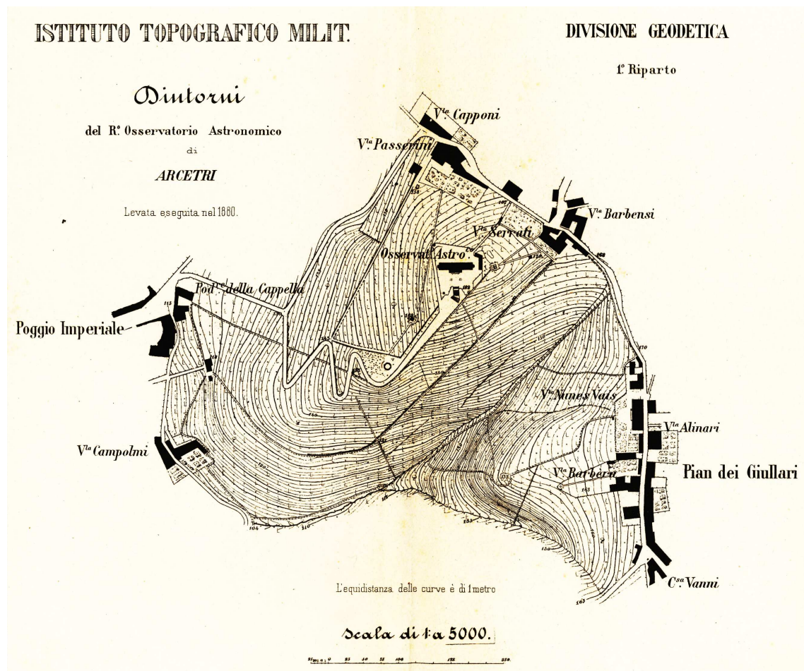
Figure 18: Arcetri Observatory and surrounds in 1880 (Archivio Storico INAF-Osservatorio Astrofisico di Arcetri). The circular wall of the 1869 pavilion still existed, but was never put into use for the magnetic instruments (after Bianchi et al., 2011).
