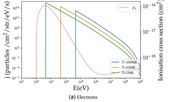
(a) Electrons
