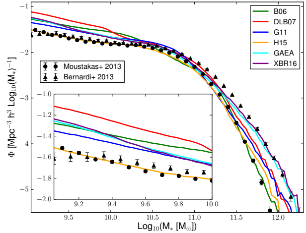
Figure 2. The galaxy stellar mass function predicted by the six models used in our study, compared to observational measurements by Moustakas et al. (2013, circles) and Bernardi et al. (2013, triangles), both based on SDSS. The inset shows a zoom on the low-mass end.
