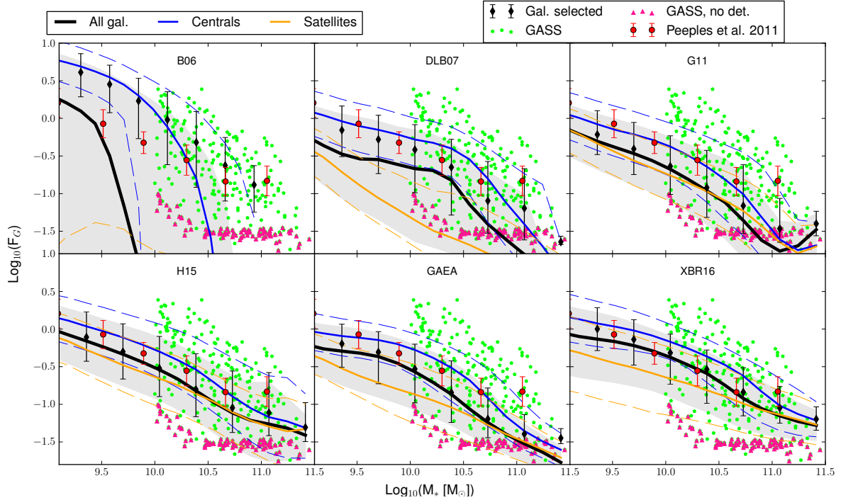
Figure 5. The gas fraction F_G = M_{cold}/M_* of model galaxies as a function of their stellar mass, compared to observational measurements by Catinella et al. (2013, green pentagons and pink triangles), and Peeples & Shankar (2011, red circles with error bars). Lines (solid and dashed), shaded region and diamonds with error-bars have the same meaning as in Fig. 4.
